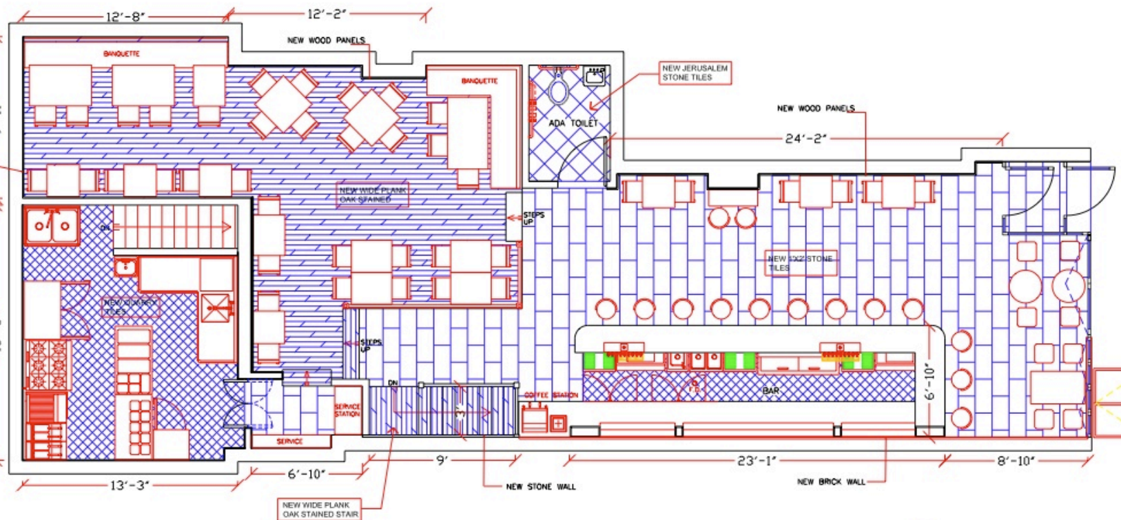
Floorplan
